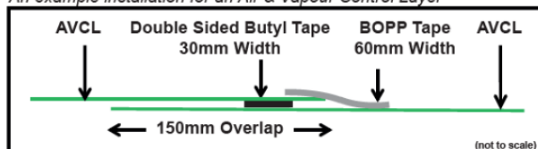
An example installation for an Air & Vapour Control Layer
